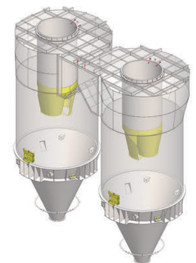
新型旋风筒内筒及旋风收尘器 New inner cylinder of cyclone and cyclone dust collector
